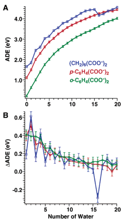
Figure 3. Comparisons of the adiabatic electron detachment energies (ADE) of ^{-}\text{O}_2\text{C}(\text{CH}_2)_6\text{CO}_2^{-}(\text{H}_2\text{O})_n ( n = 0-20 ) with those of p\text{-C}_6\text{H}_4(\text{CO}_2^{-})_2 ( n = 0-20 ) and o\text{-C}_6\text{H}_4(\text{CO}_2^{-})_2 ( n = 0-20 ). (A) The ADE as a function of solvent number ( n ). (B) Differential ADE, defined as \Delta\text{ADE} = \text{ADE}(n) - \text{ADE}(n - 1) . Blue curve, hydrated suberate; red curve, hydrated p -benzene dicarboxylate; green curve, hydrated o -benzene dicarboxylate.
