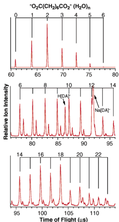
Figure 1. Typical mass spectra of ^{-}\text{O}_2\text{C}(\text{CH}_2)_6\text{CO}_2^{-}(\text{H}_2\text{O})_n from electro-spray ionization of a substrate solution, that were optimized for three mass ranges. \text{H}[\text{DA}]^{-} and \text{Na}[\text{DA}]^{-} indicated the singly charged protonated and sodiated substrate ion pairs, respectively.
