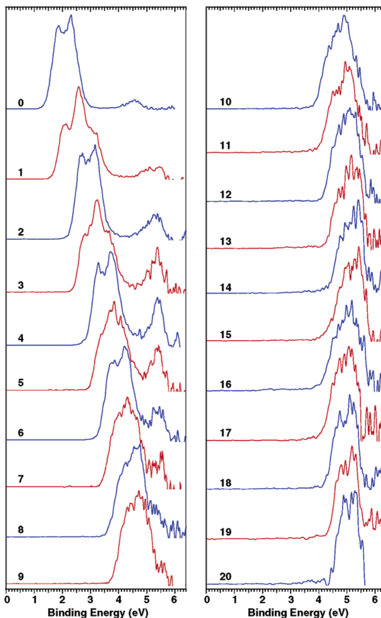
Figure 2. Photoelectron spectra of {}^{-}\text{O}_2\text{C}(\text{CH}_2)_6\text{CO}_2{}^{-}(\text{H}_2\text{O})_n ( n = 0\text{--}20 ) at 193 nm (6.424 eV).
